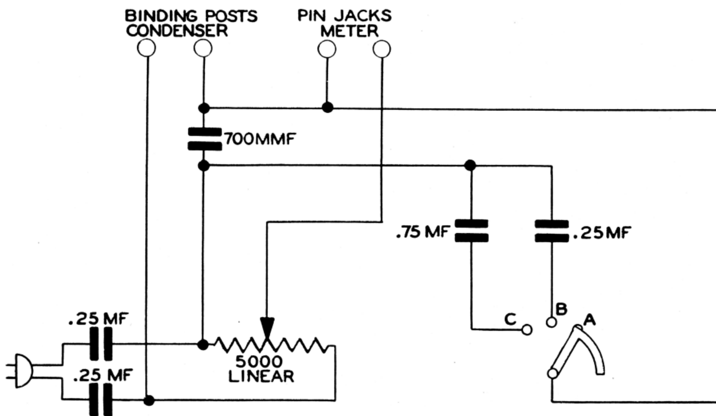
PHILCO MODEL 010 CONDENSER TESTER (SCHEMATIC DIAGRAM)
