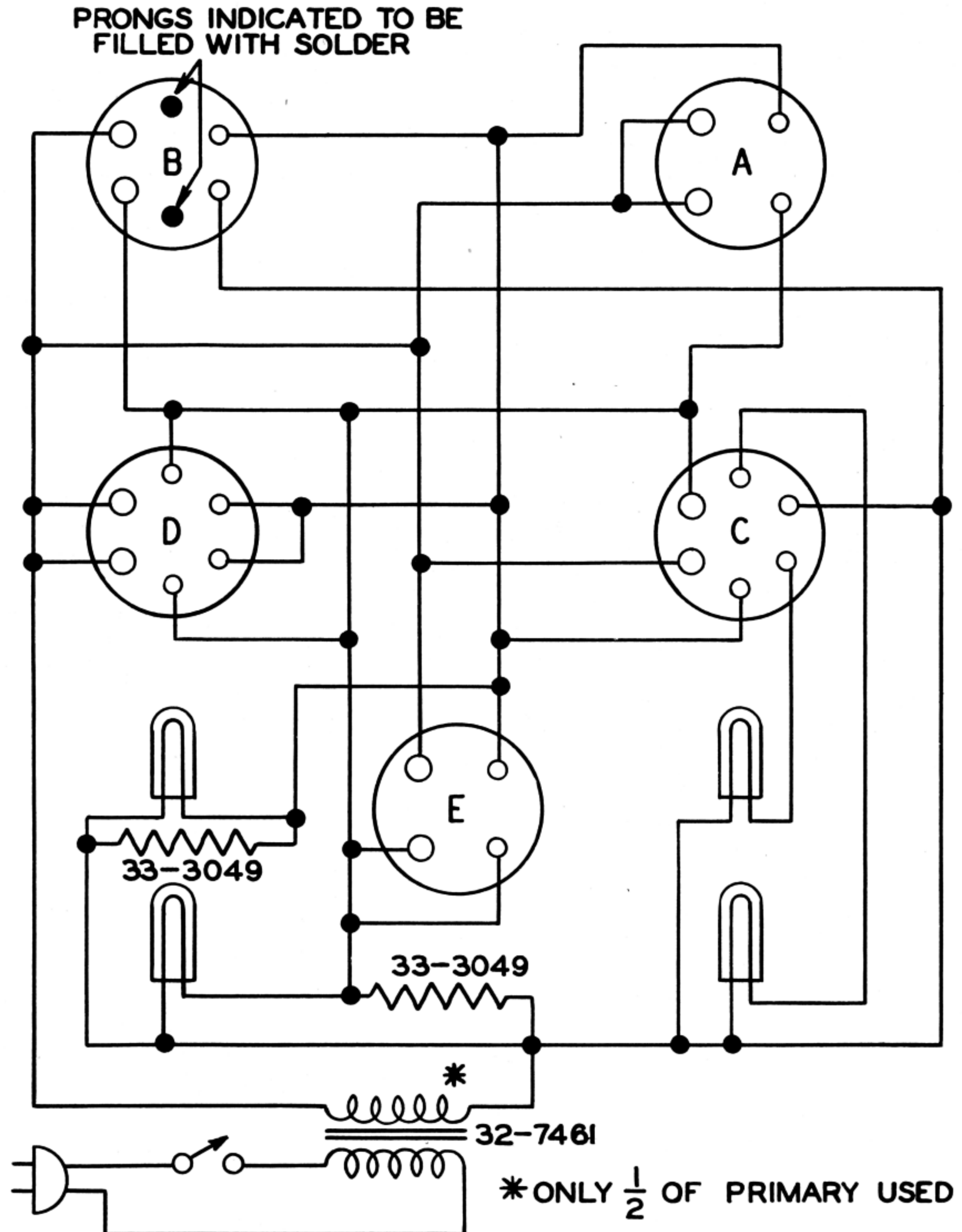
PHILCO MODEL 013 VIBRATOR TESTER (SCHEMATIC DIAGRAM)
