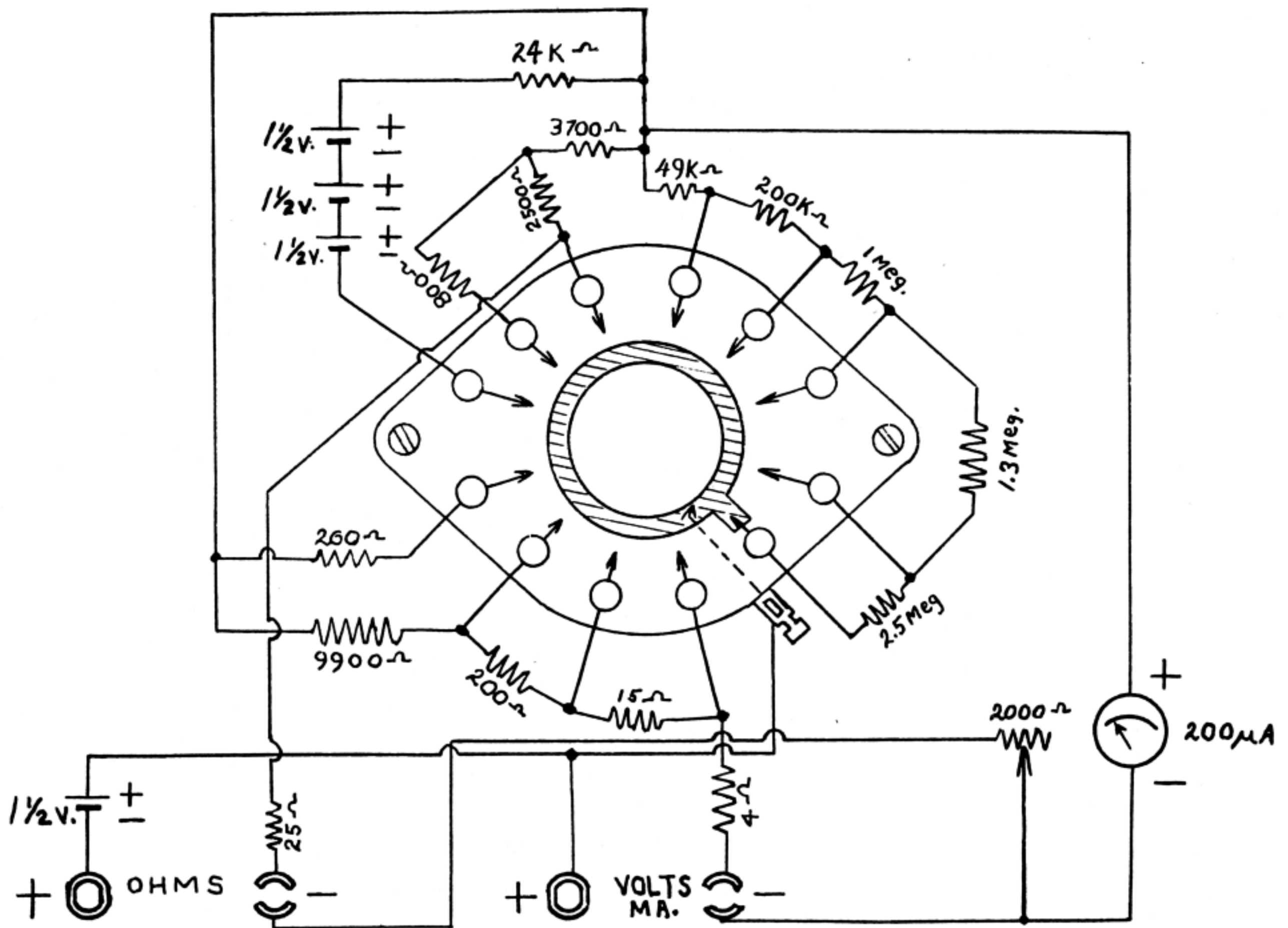
PHILCO MODEL 023 VOLT-OHM-MILLIAMMETER (SCHEMATIC DIAGRAM)
