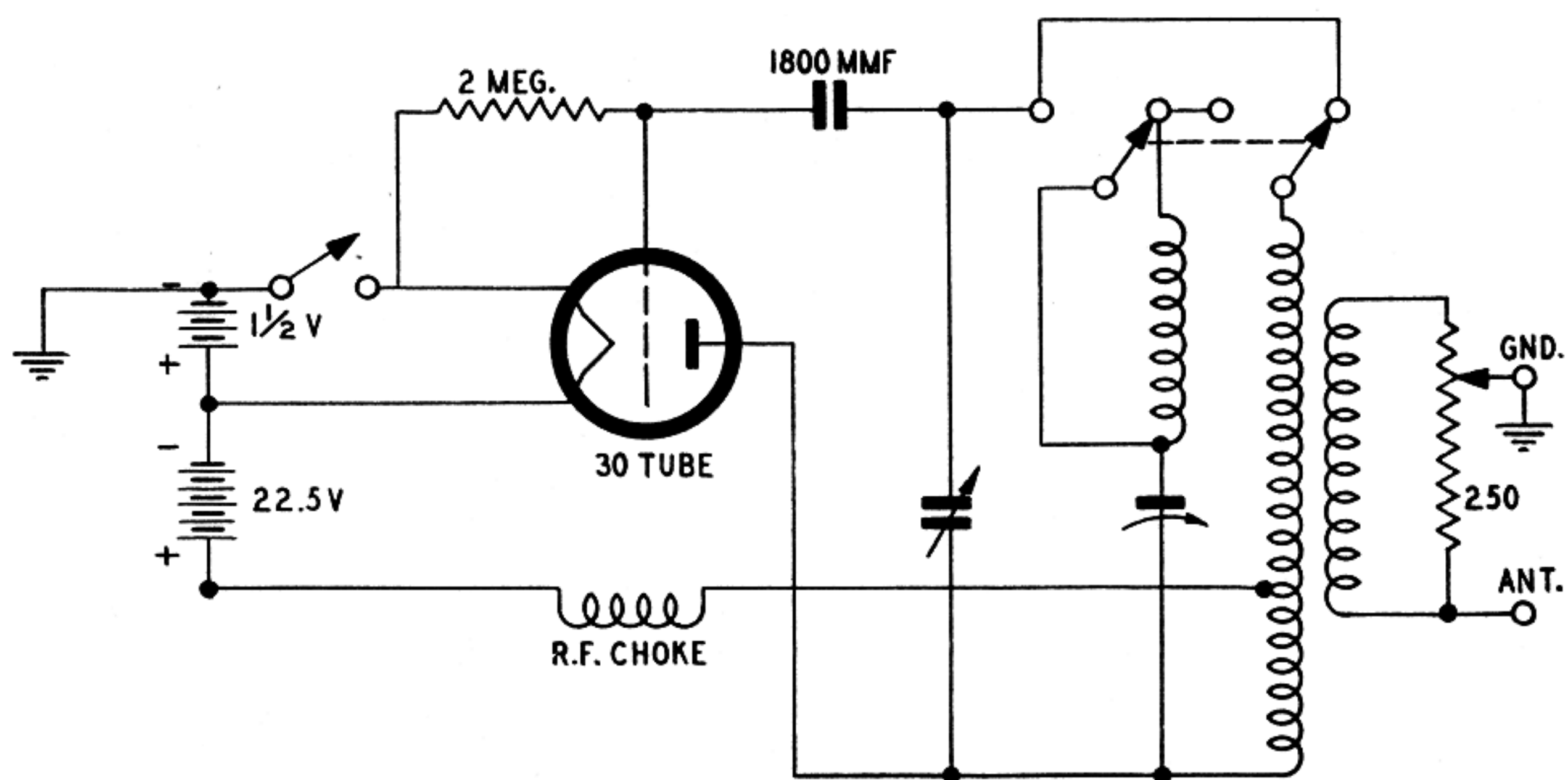
PHILCO MODEL 024 SIGNAL GENERATOR (SCHEMATIC DIAGRAM)
